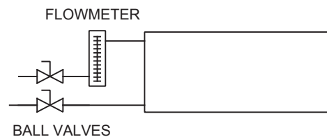
PLUMBING SCHEMATIC
