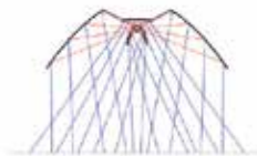
Surna Reflector Light Dispersion Pattern
